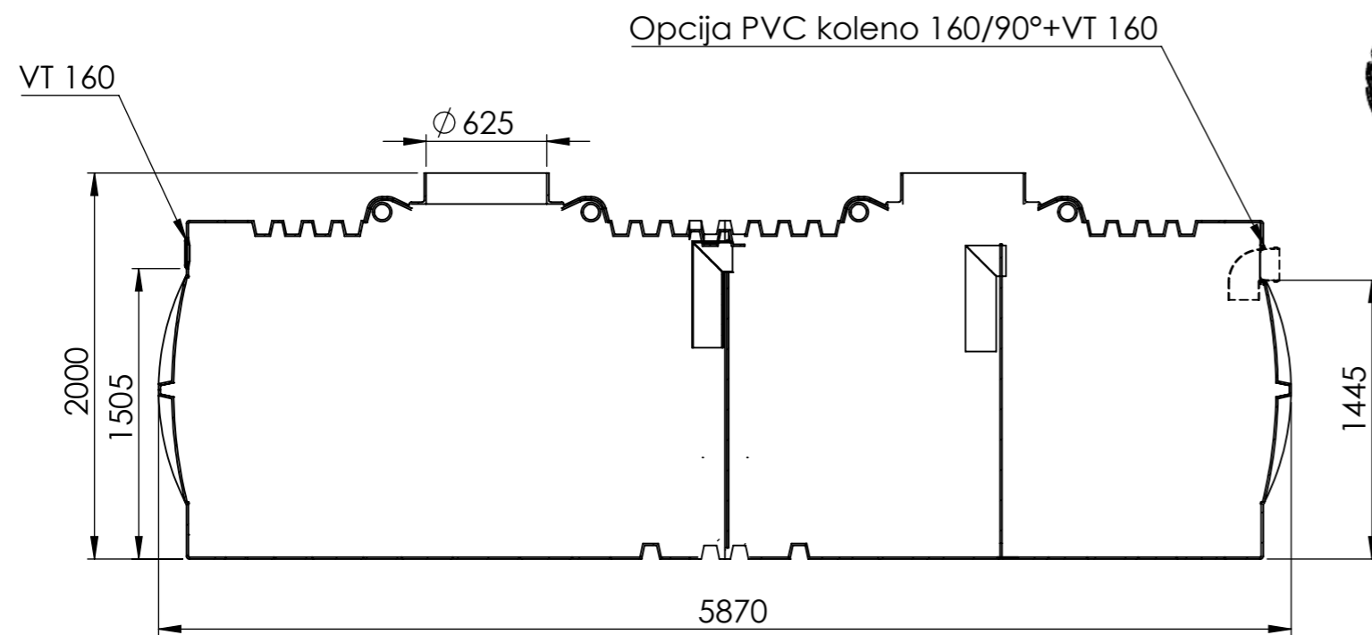
SECTION C-C SCALE 1 : 35
